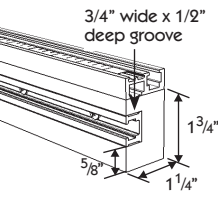
Fig. 11 T-Track Fence
